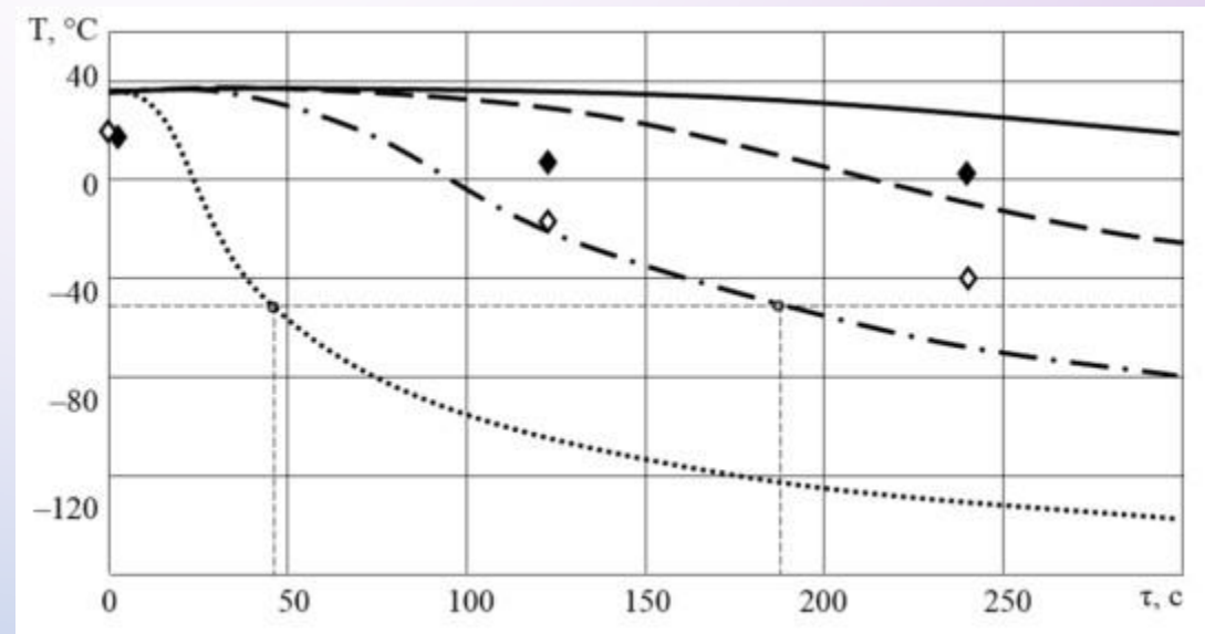
Calculated temperature field of cryo in biological objects
